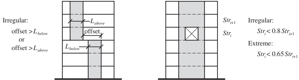
Type 4. In-Plane Discontinuity
