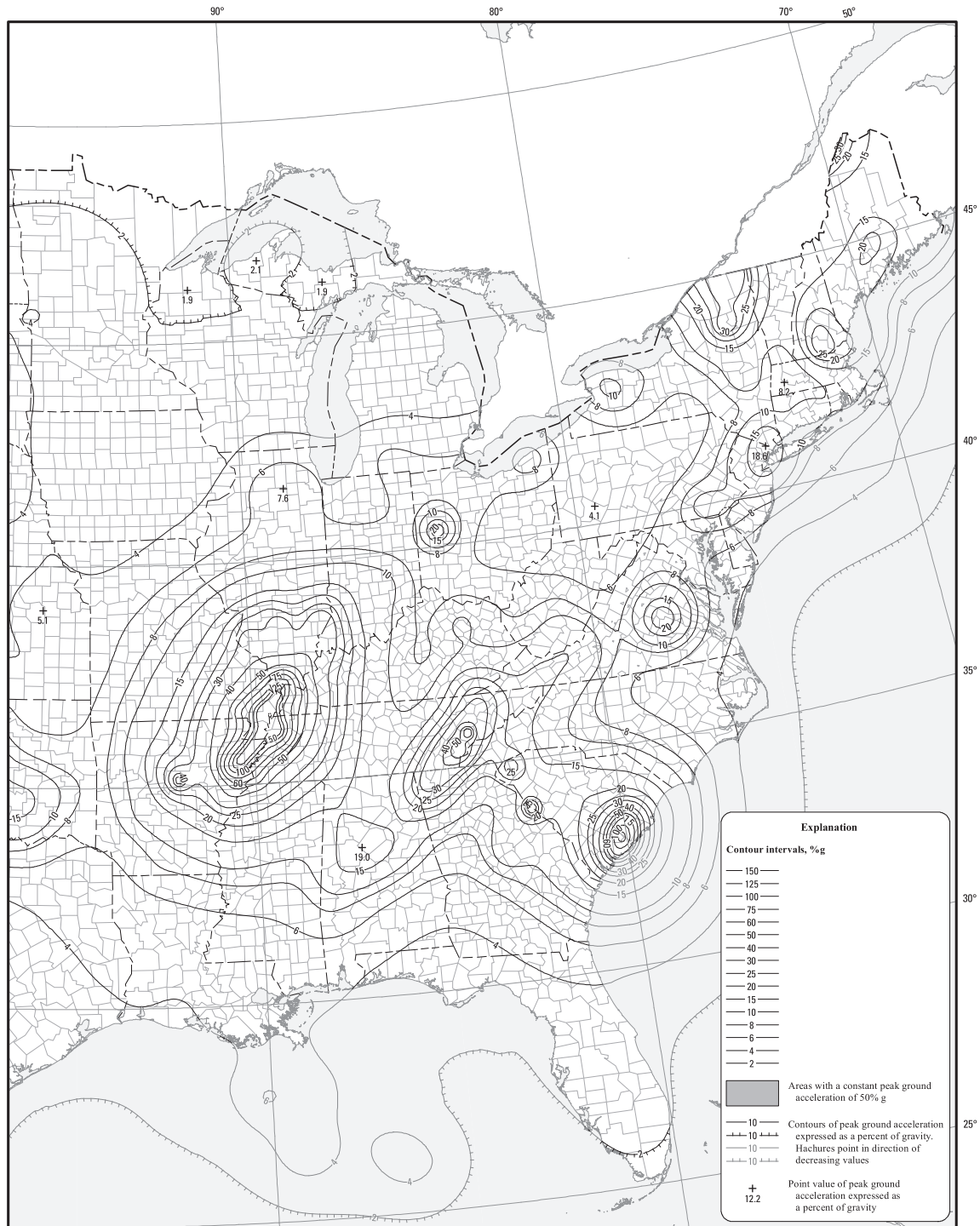
FIGURE 22-9 (Continued). Maximum Considered Earthquake Geometric Mean ( MCE_G ) PGA, %g, for the Conterminous United States
