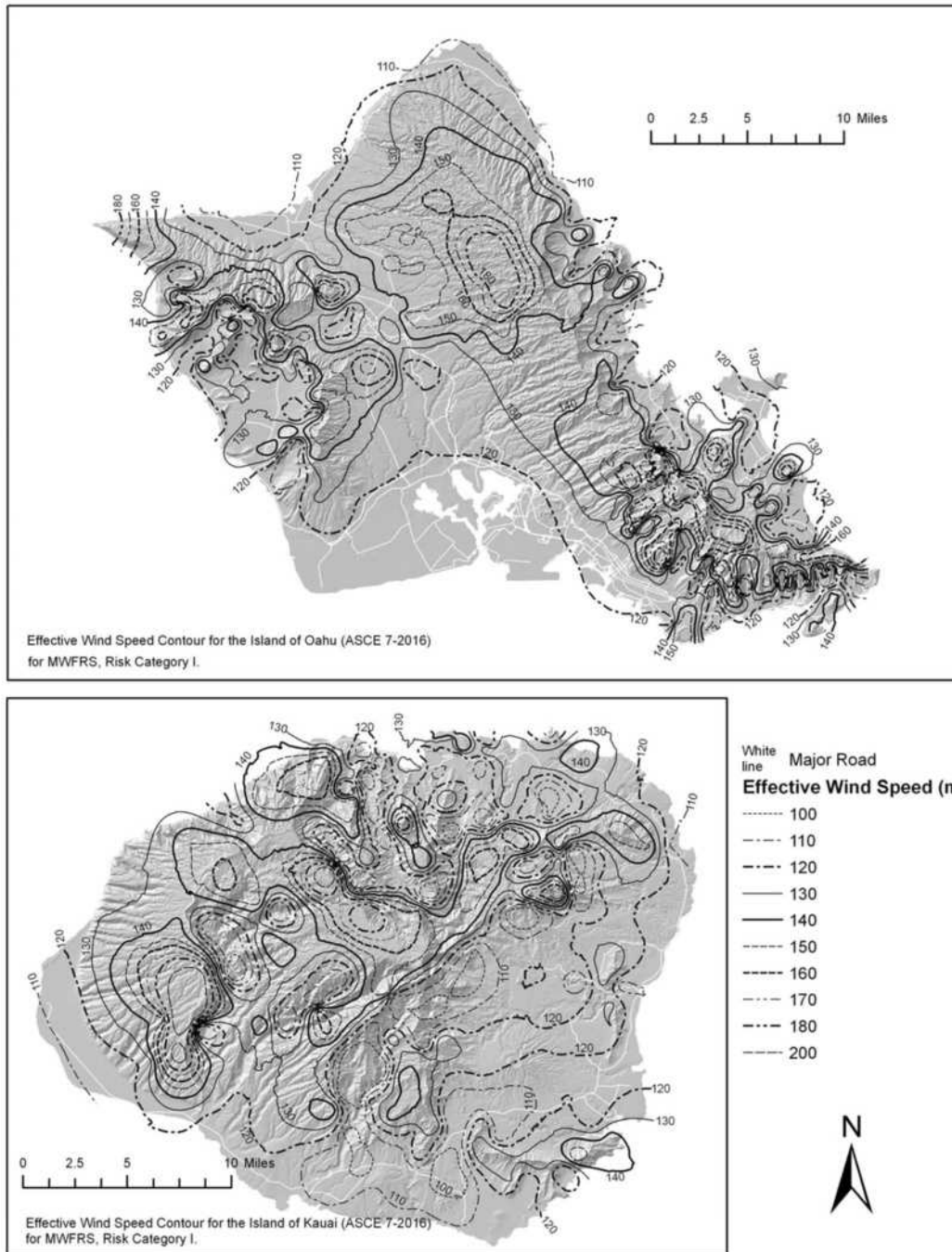
FIGURE 26.5-2A (Continued). Basic Wind Speeds for Risk Category I Buildings and Other Structures: Hawaii
