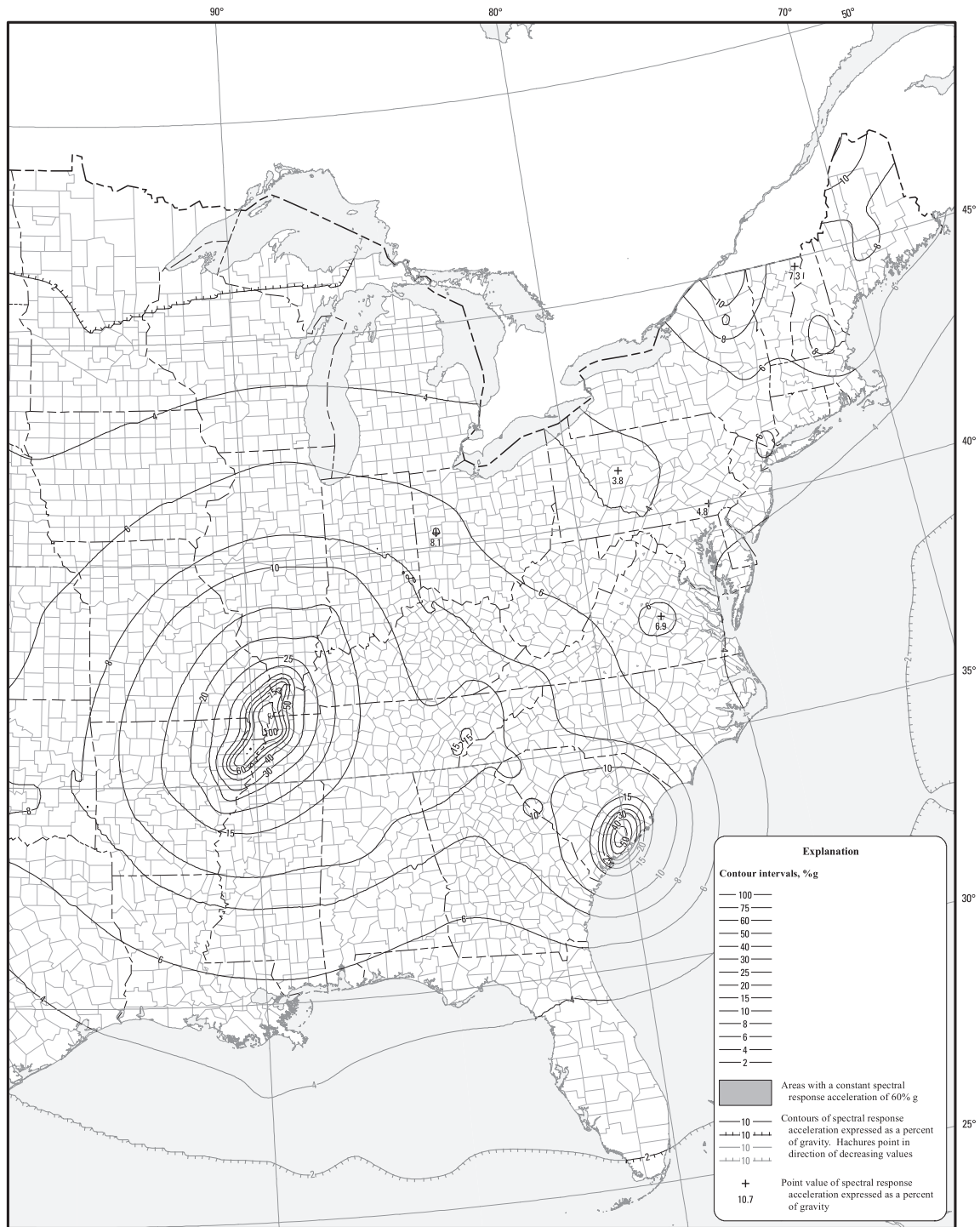
FIGURE 22-2 (Continued). S_1 Risk-Targeted Maximum Considered Earthquake ( MCE_R ) Ground Motion Parameter for the Conterminous United States for 1.0-s Spectral Response Acceleration (5% of Critical Damping)
