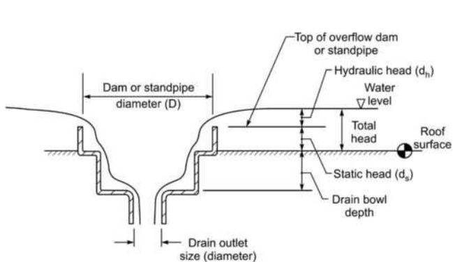
FIGURE C8.3-1 Schematic Cross Section of Secondary (Overflow) Roof Drain and Total Head ( d_s + d_h ). Drain Debris Guard (Strainer) and Ring Clamp (Gravel Stop) Not Shown for Clarity
