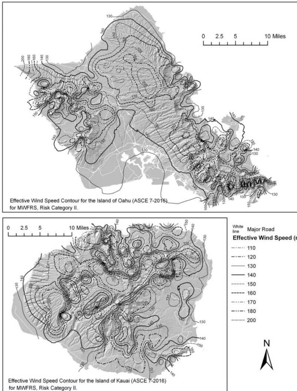
FIGURE 26.5-2B (Continued). Basic Wind Speeds for Risk Category II Buildings and Other Structures: Hawaii
